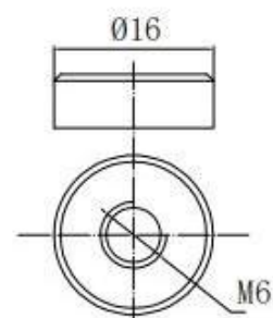
Terminal Dimensions
