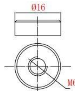
Terminal Dimensions
