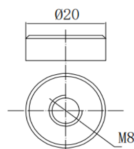
Terminal Dimensions
