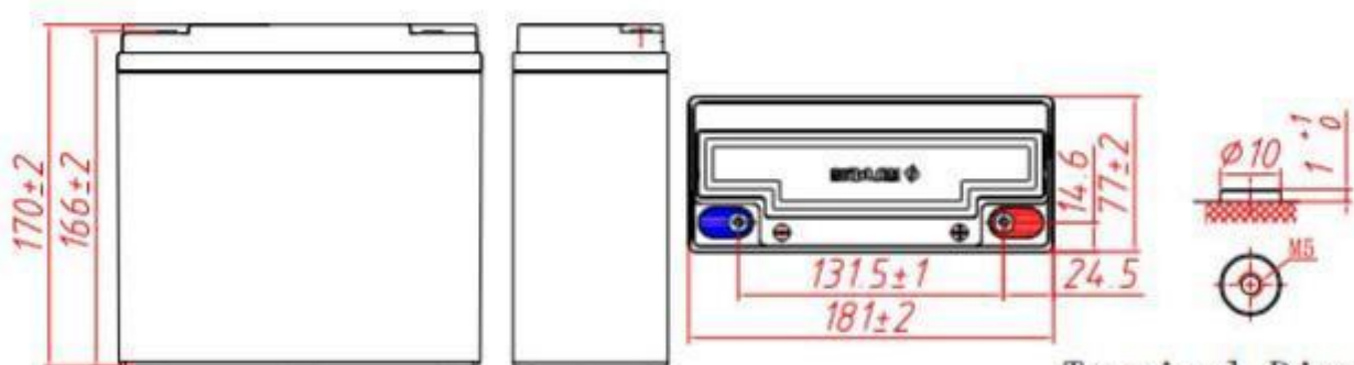
Terminal Dimensions
