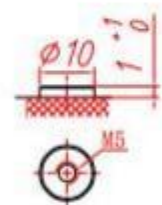
Terminal Dimensions
