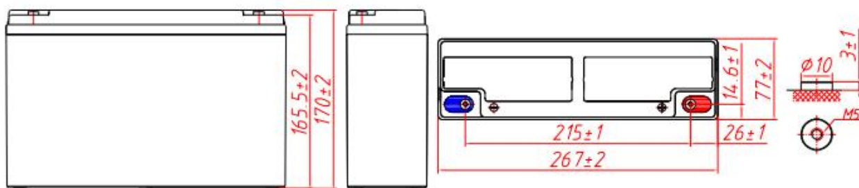
Terminal Dimensions
