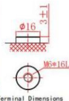
Terminal Dimensions
