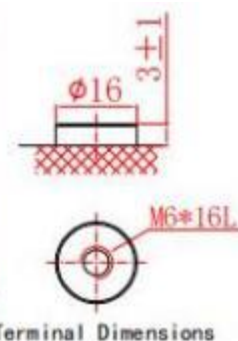
Terminal Dimensions
