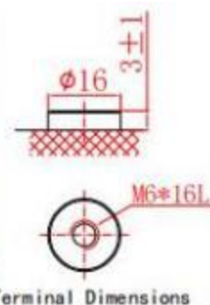
Terminal Dimensions
