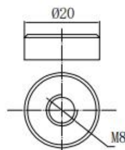
Terminal Dimensions
