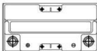
Terminal Dimensions
