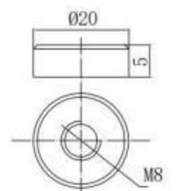
Terminal Dimensions
