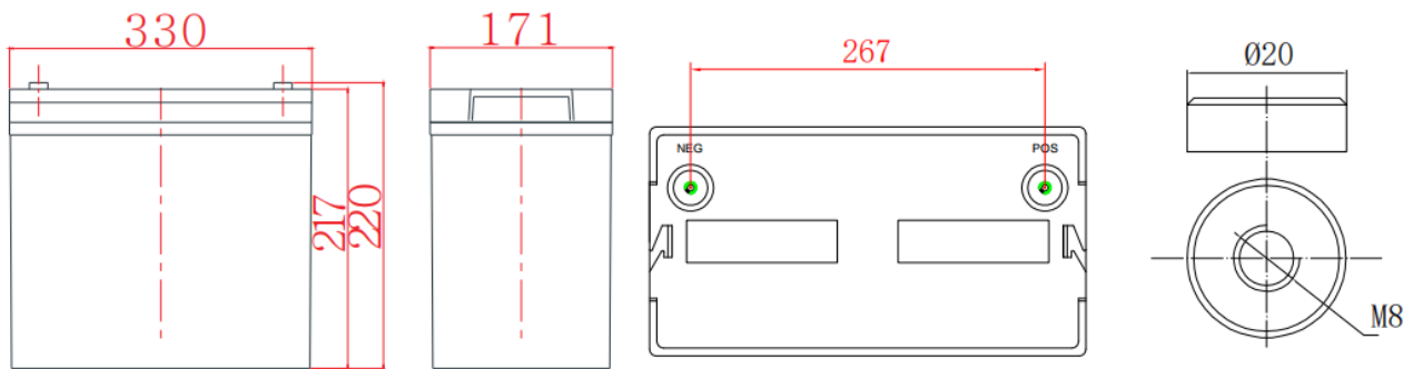
Terminal Dimensions
