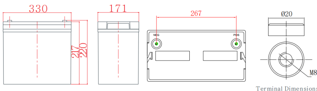
Terminal Dimensions
