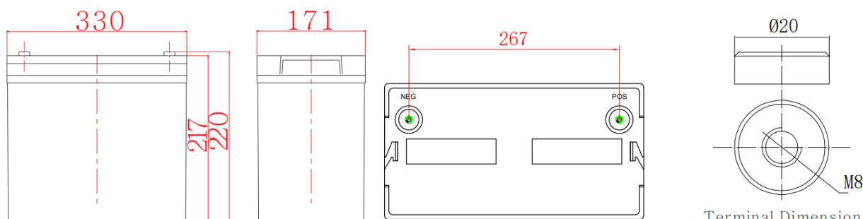
Terminal Dimensions
