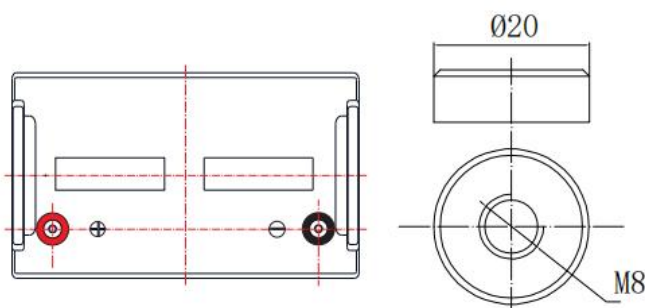
Terminal Dimensions
