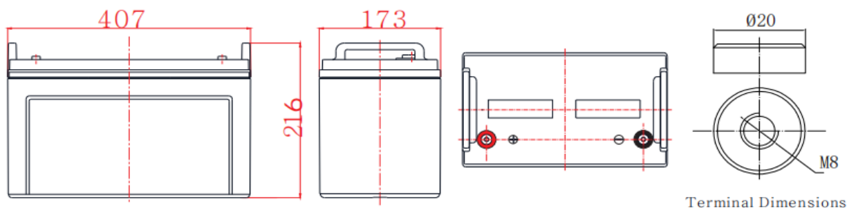
Terminal Dimensions
