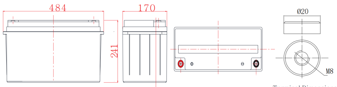
Terminal Dimensions
