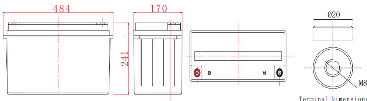
Terminal Dimensions
