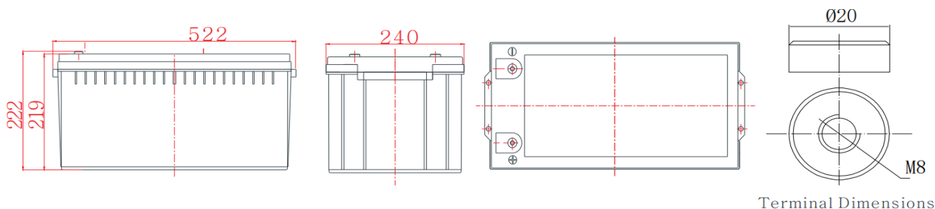
Terminal Dimensions
