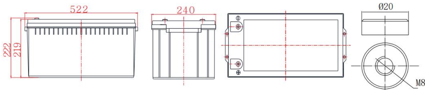
Terminal Dimensions
