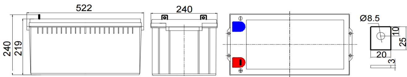
Terminal Dimensions
