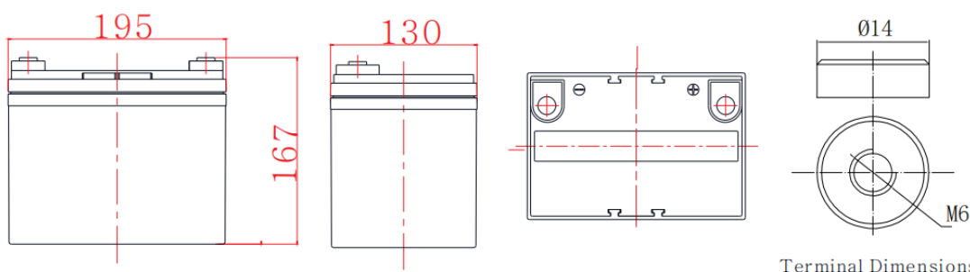
Terminal Dimensions
