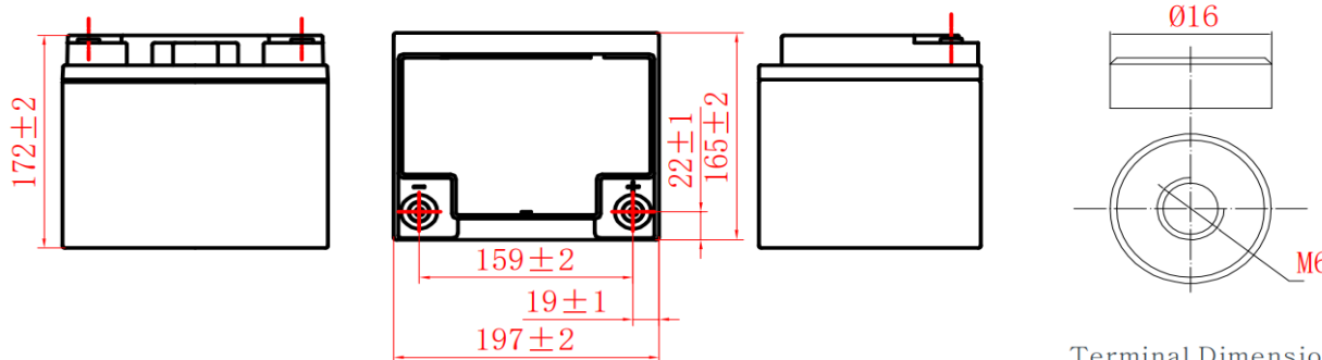
Terminal Dimensions
