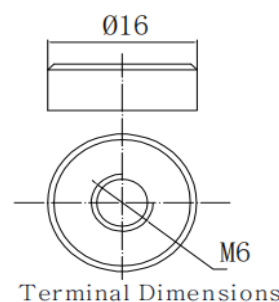
Terminal Dimensions
