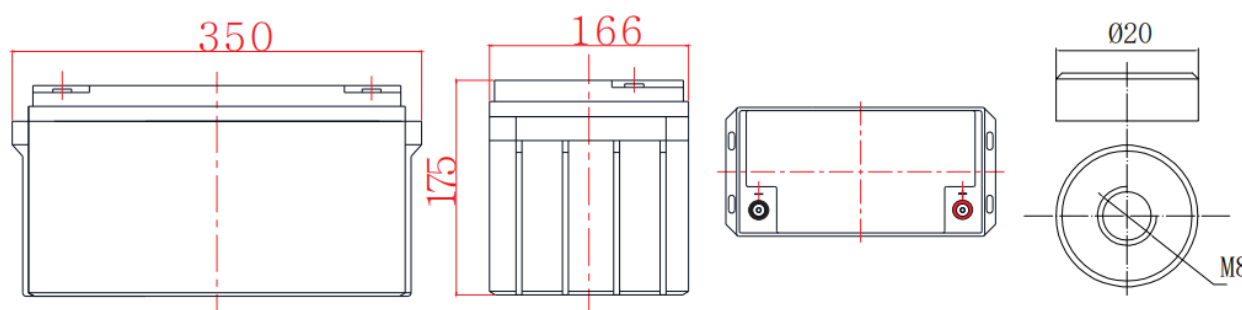
Terminal Dimensions
