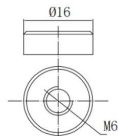
Terminal Dimensions
