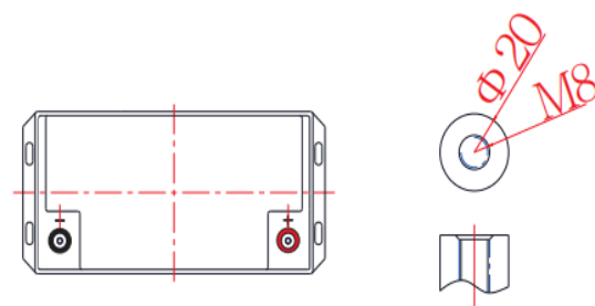
Terminal Dimensions
