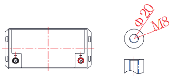
Terminal Dimensions
