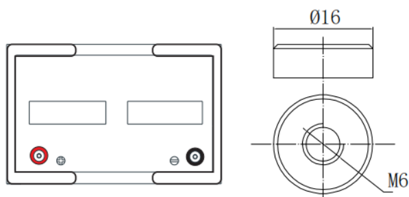
Terminal Dimensions
