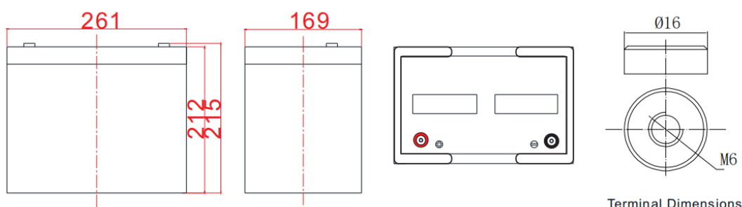
Terminal Dimensions
