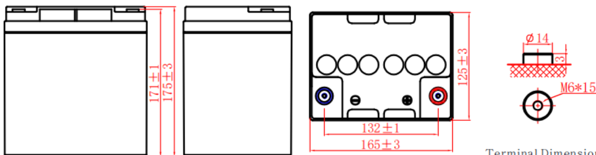
Terminal Dimensions
