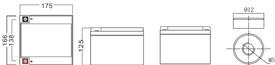
Terminal Dimensions
