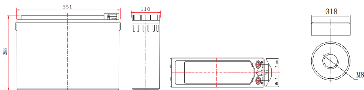
Terminal Dimensions
