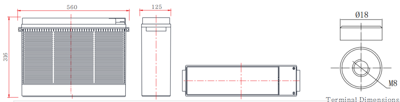
Terminal Dimensions
