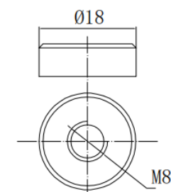
Terminal Dimensions
