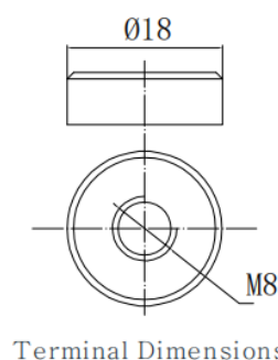
Terminal Dimensions
