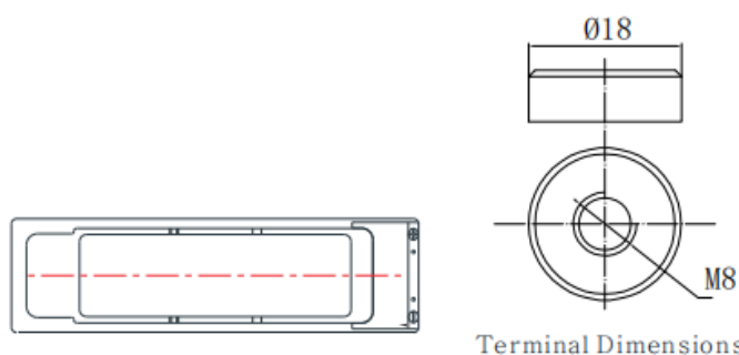
Terminal Dimensions
