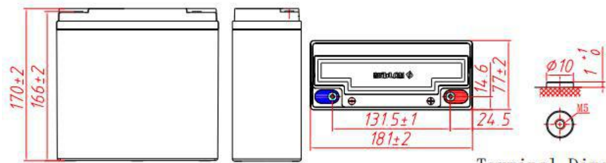
Terminal Dimensions
