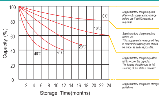
Storage Characteristics
