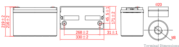
Terminal Dimensions
