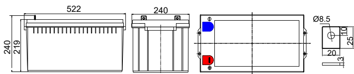
Terminal Dimensions
