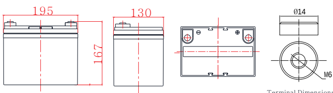
Terminal Dimensions
