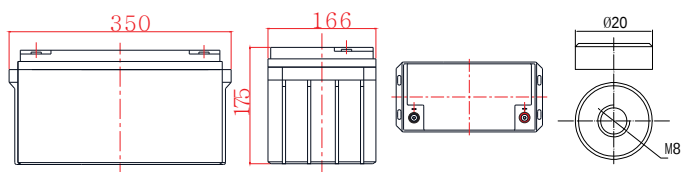
Terminal Dimensions
