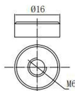
Terminal Dimensions
