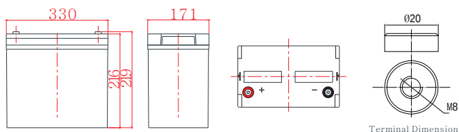
Terminal Dimensions
