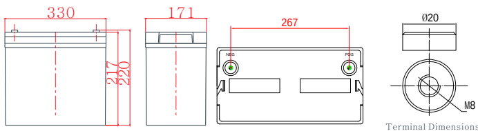
Terminal Dimensions
