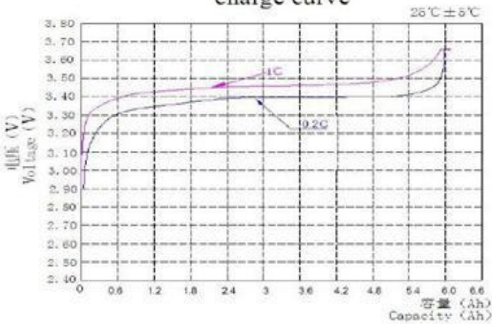
充电曲线图 charge curve
